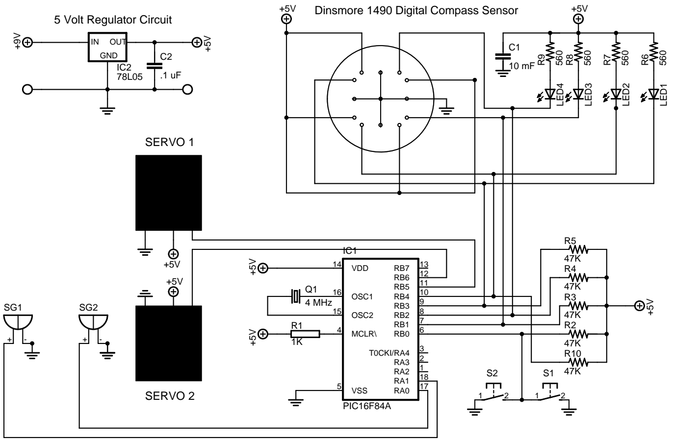
Digital Compass Car Circuit
